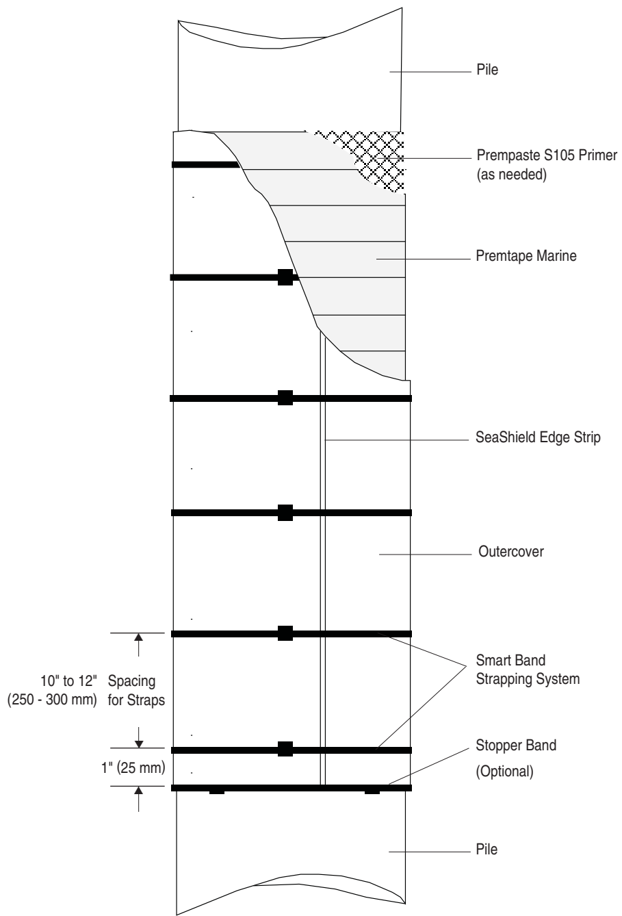
Elevation View
