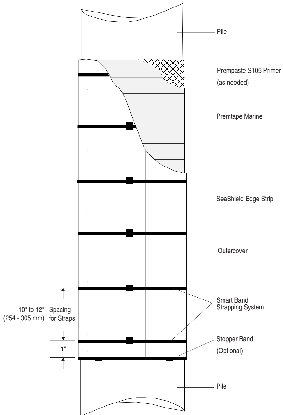
Elevation View
