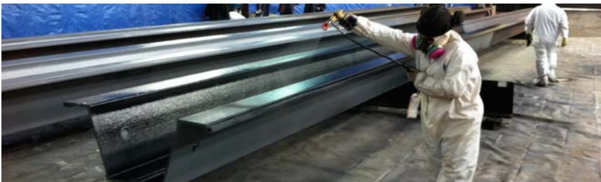
Premier Rigspray being applied to steel sheet piles with an airless spray unit.
