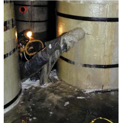
Structurally repaired timber piles with rebar, concrete and translucent SeaShield Fiber-Form fiberglass pile jackets.
